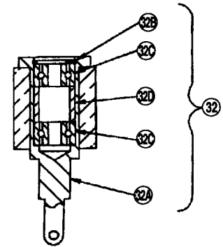
Driver Magnet Holder and Bearing Assembly
